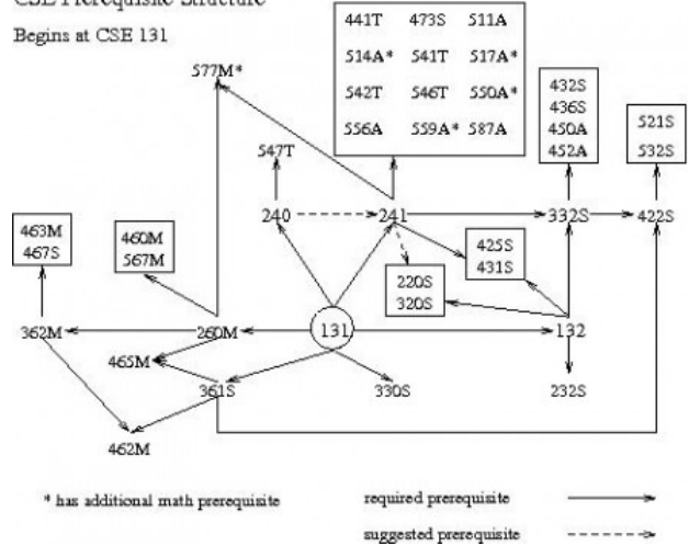
CSE Prerequisite Structure
